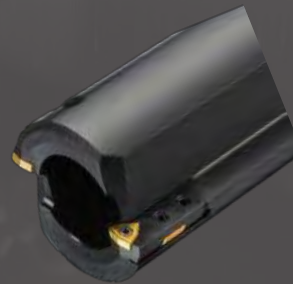
T-Max U Trepan Large dia holes where power is limited
